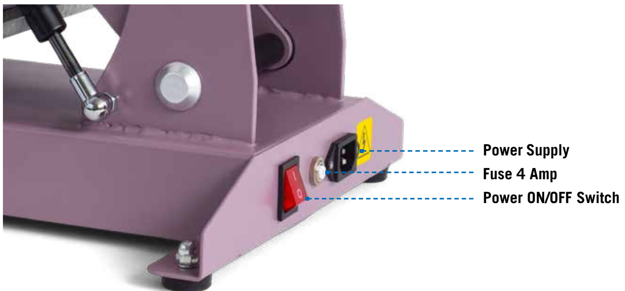
Rear view of heat press
